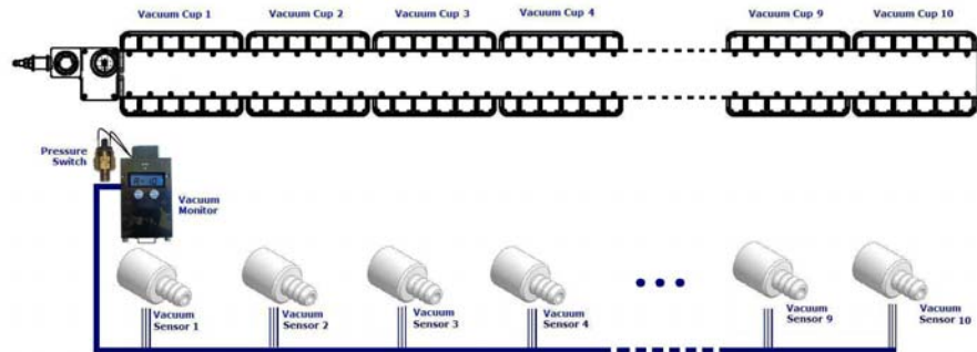
Flex Track Vacuum Monitoring System Layout
