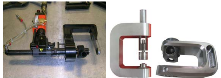
Power-Feed & Hand-Held C-Clamps
